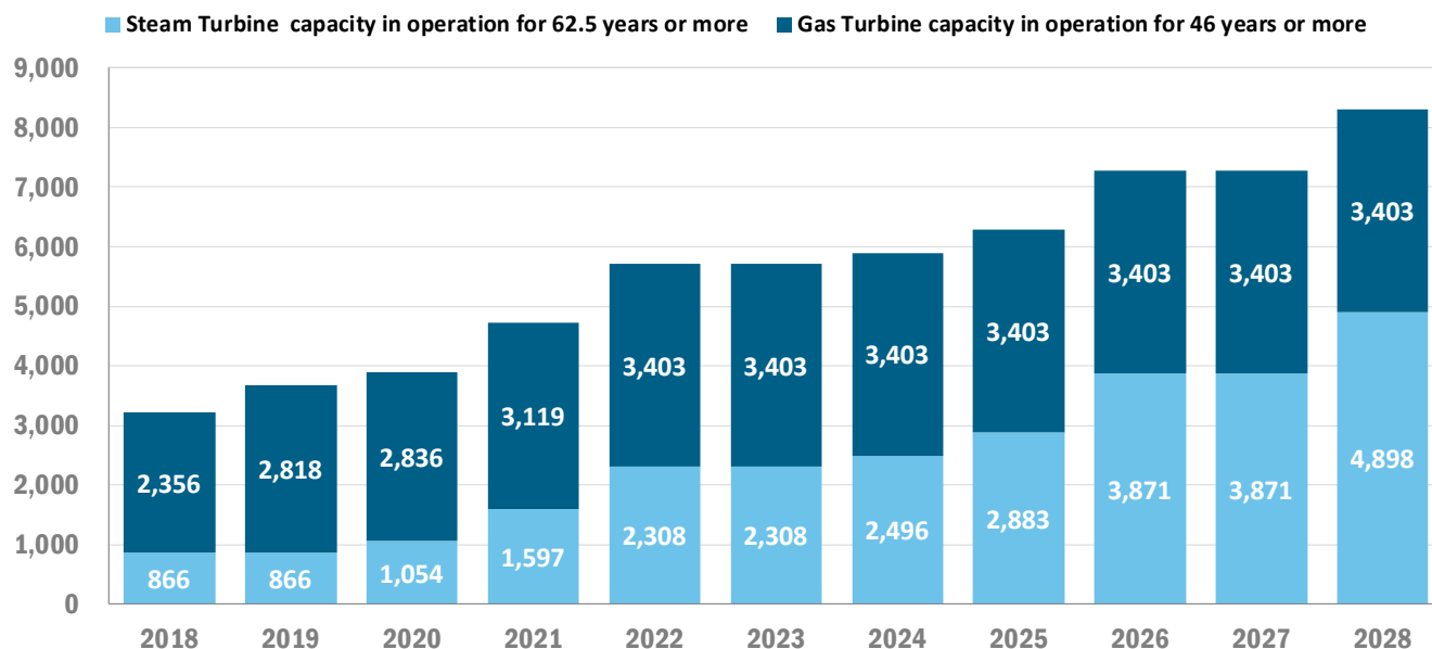
Figure 1: Aging Fossil Fuel Nameplate Capacity: Gas Turbines & Steam Turbines Nearing Retirement
